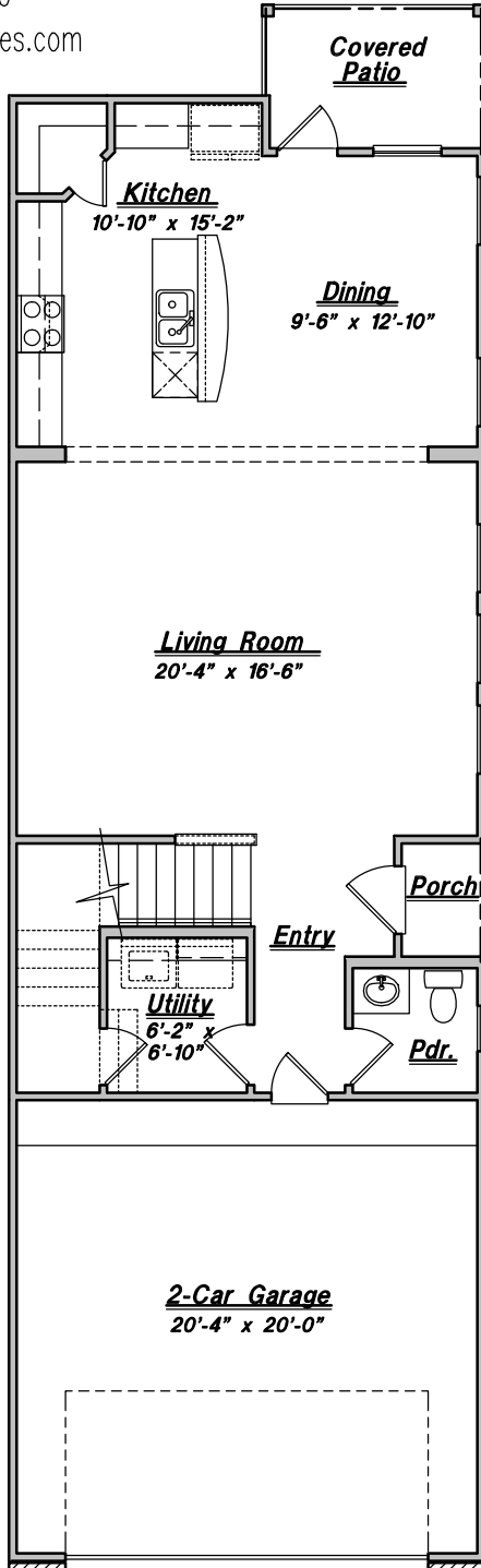
FIRST FLOOR PLAN Plan CH-2000
