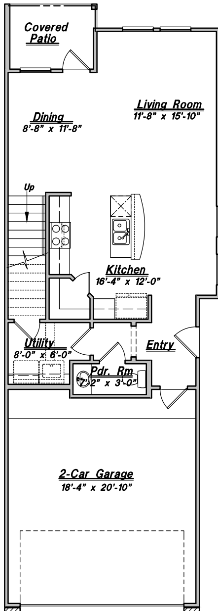
FIRST FLOOR PLAN Plan CH-1600
