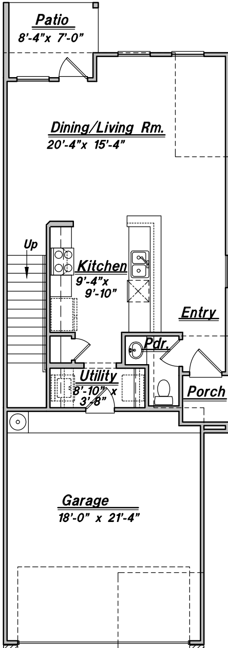
FIRST FLOOR PLAN Plan 1556
