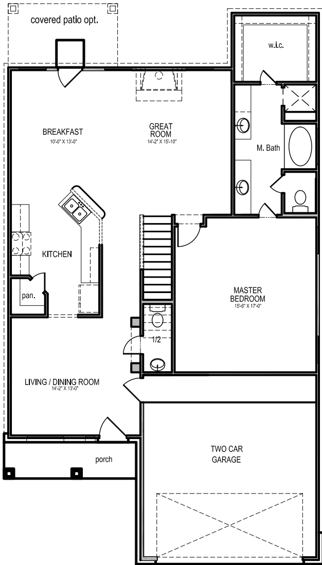
1ST FLOOR
